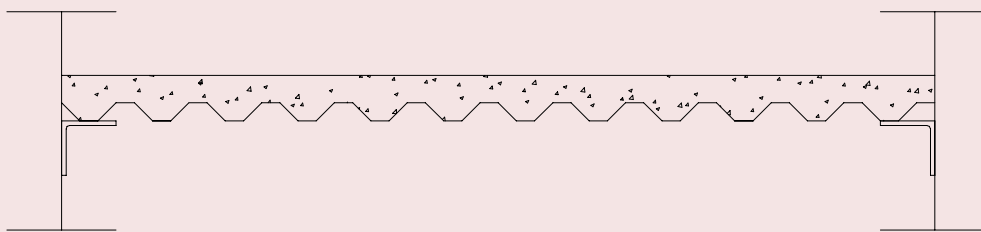
Figure 4. Crossover cross-section. Note: transverse members allow the deck to run parallel to the girders as shown.
