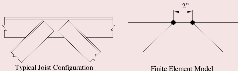
Figure 3. Joist panel point eccentricity.
