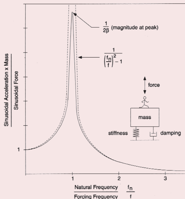
Figure 1. Resonance response (Figure 1.3 of the AISC/CISC design guide).
